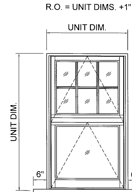
EXTERIOR ELEVATION OF SERIES 4000 IN-LINE FOLD-UP OUT WINDOW UNIT WITH SILL
